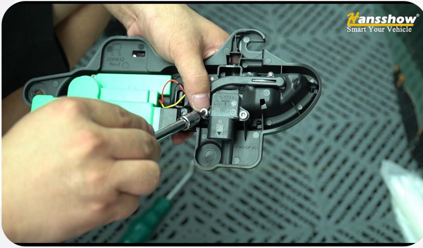
15. Install the original vehicle module onto the power door handle
