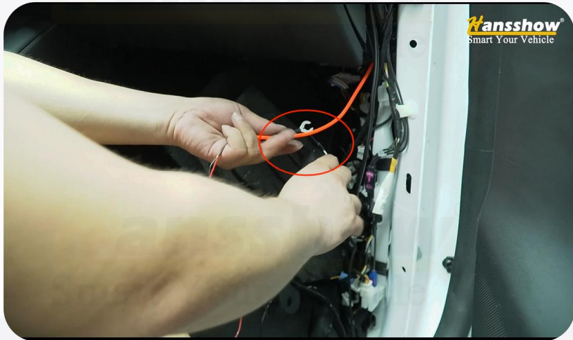
47. Wrap the positive and negative wires with the threading tool and pull them to the battery location.
