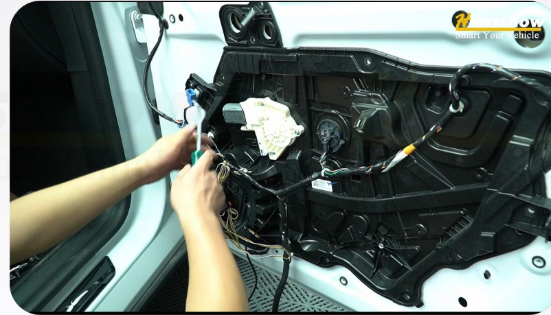
10. Pry open the connector of the wires inside the interior trim panel and unplug it
