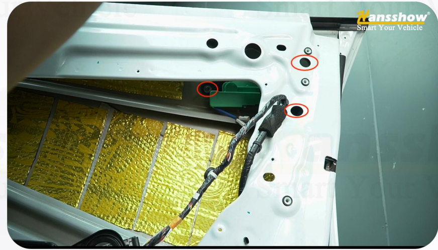
16. Tighten the three securing screws
