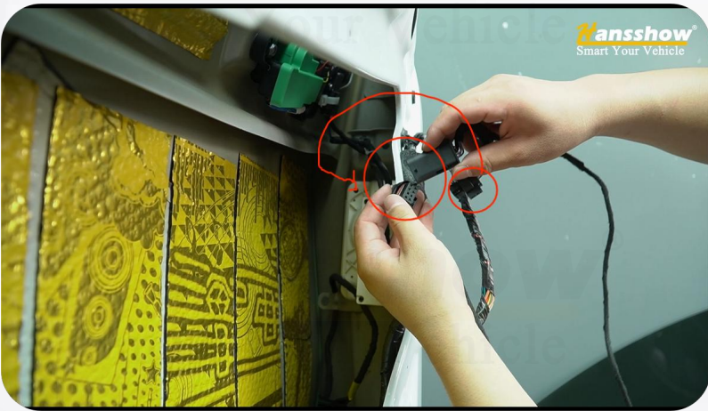
19. Connect the adapter plug to the original vehicle plug, and connect the other plug to the original vehicle lock block
