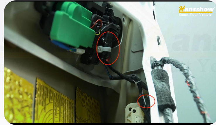
18. After plugging in the connector, remove the plug of the original vehicle lock block
