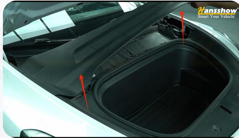
42. Remove the cover of the frunk
