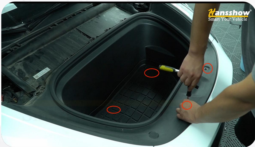
43. Loosen these four screws (after removing the pad, there are two screws inside)
