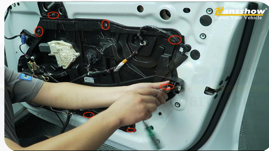
8. Loosen the surrounding screws
