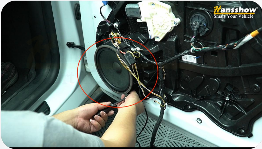
9. Loosen the screws around the speaker
