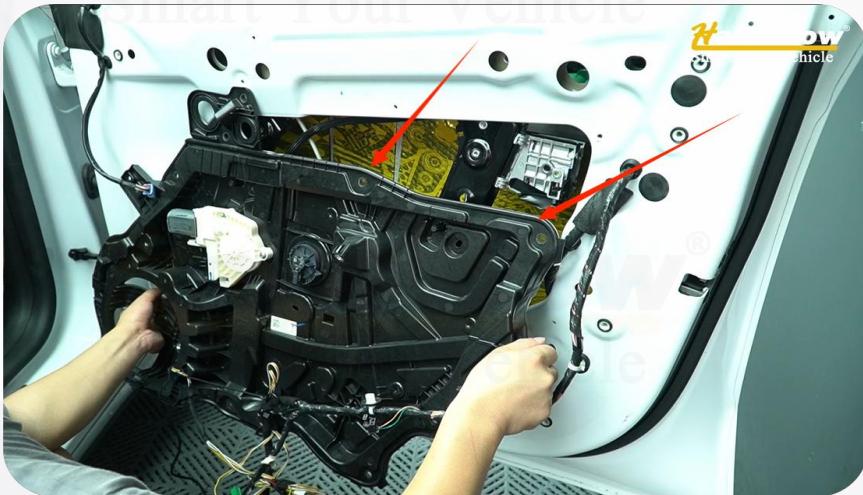
11. Remove the interior trim panel
