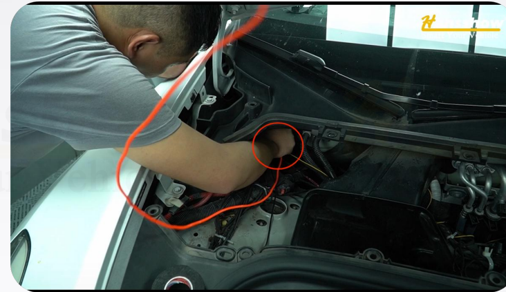
46. Guide the threading tool along the rubber grommet to the passenger footwell area
