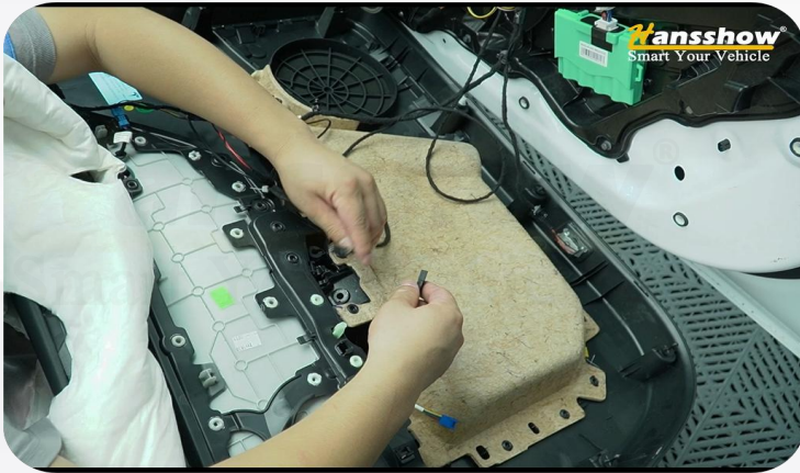
25. Restore the original connection of the wires in the car door
