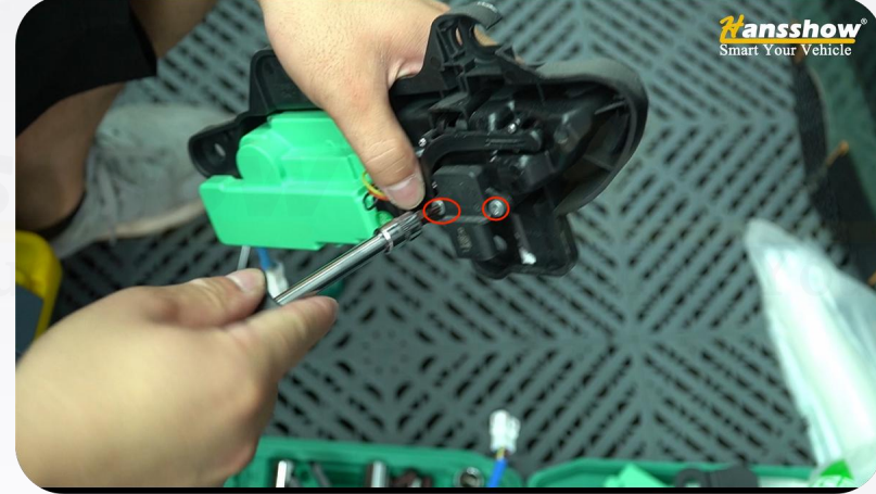
14. Loosen these two screws to remove the original vehicle module
