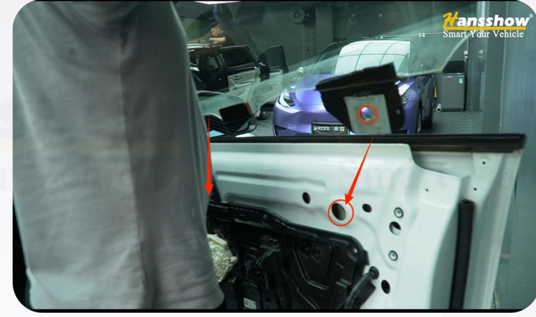
22. Align the holes with the clamp of the window regulator and tighten the screws to secure it
