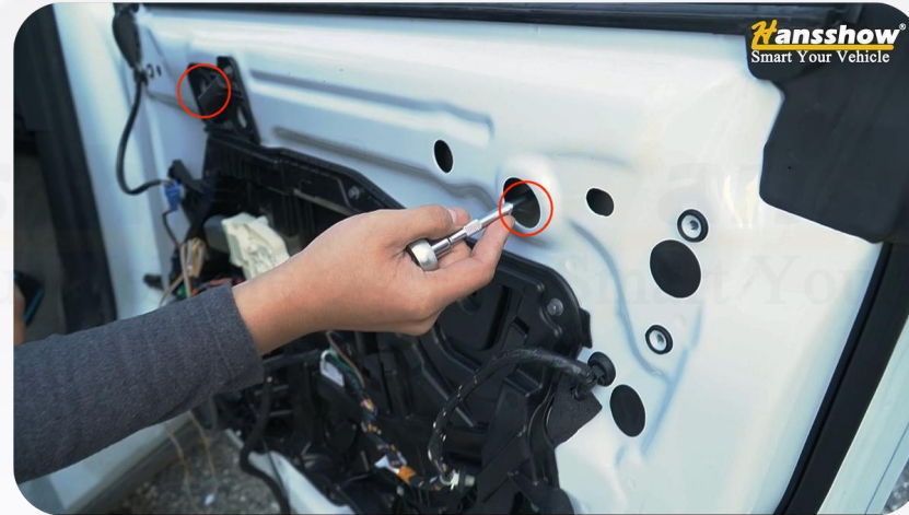
6. Loosen these two screws (with the window raised to the highest position)
