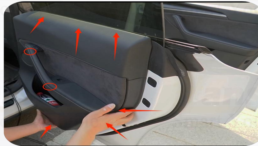
28. Loosen the two screws, pry open the clips, and lift the door upwards to remove it
