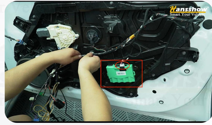
24. Attach the control box to the back using 3M adhesive, then plug in the adapter cable connector
