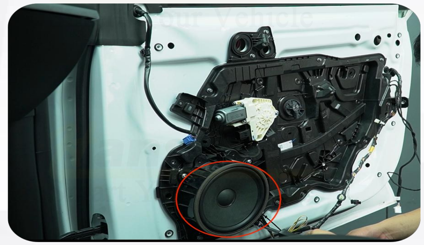
23. Secure the speaker by tightening the screws
