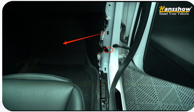
39. Pry open this clip and pull it towards the left
