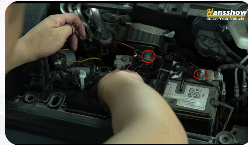
48. Secure the positive and negative wires by tightening the screws and use cable ties to secure the wire harness. Then, restore the vehicle to its original state
